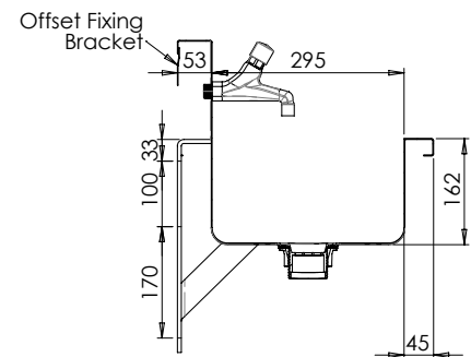
MODEL TPWDPH Section
