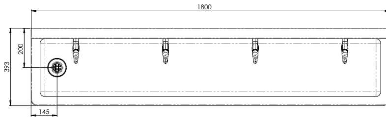
MODEL TPWDPH Plan
