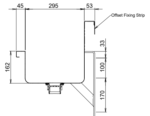
MODEL TPWD Section
