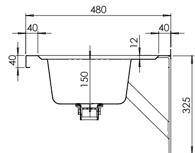
MODEL TP8I Section
