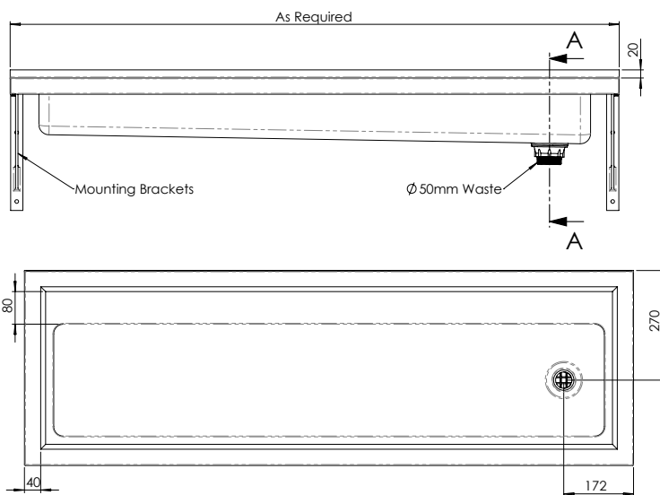
MODEL TP8I Front Elevation & Plan
