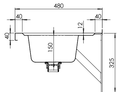
MODEL TP8F Section
