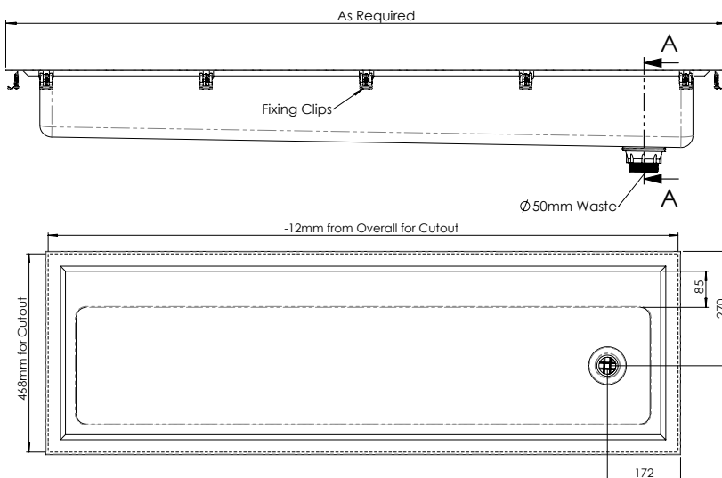
MODEL TP8I Front Elevation & Plan
