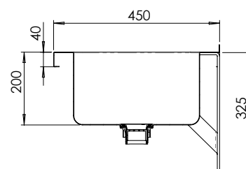
MODEL TP7F Section
