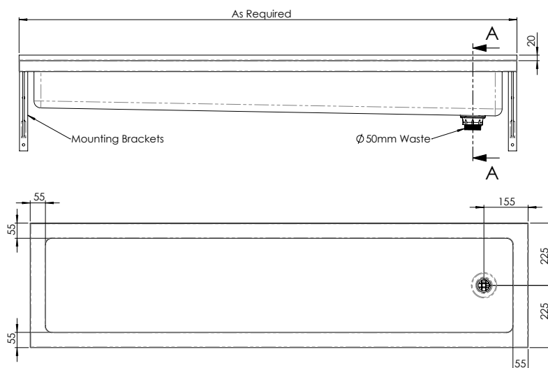
MODEL TP7I Front Elevation & Plan
