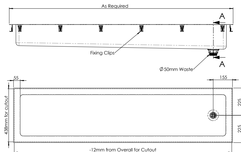
MODEL TP7I Front Elevation & Plan
