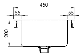
MODEL TP7I Section
