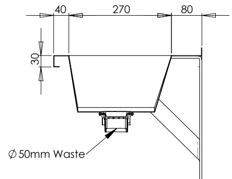
MODEL TP4 Section
