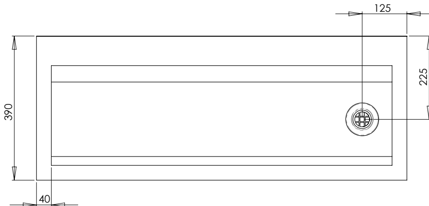
MODEL TP4 Plan
