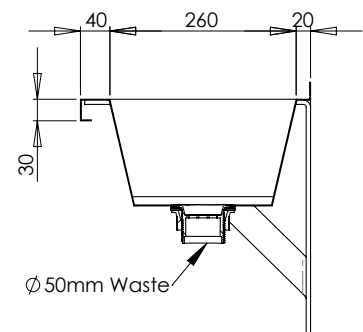
MODEL TP1 Section
