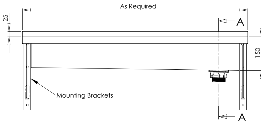
MODEL TP1 Front Elevation
