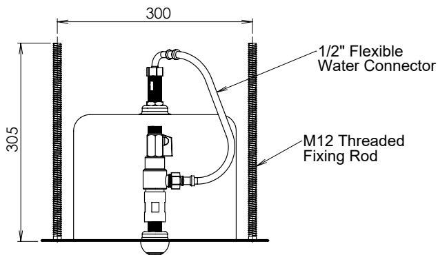
MODEL SRB Plan Elevation
