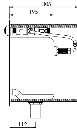
MODEL SRB Side View
