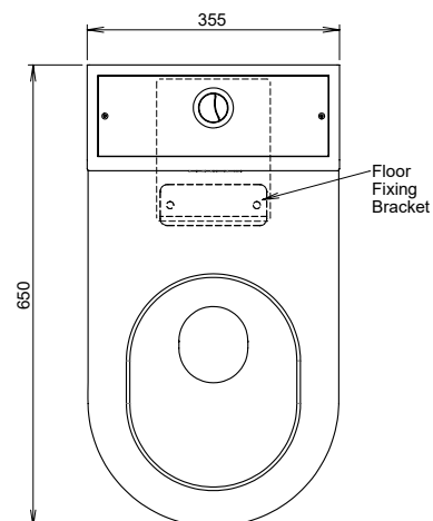
MODEL PTS Plan
