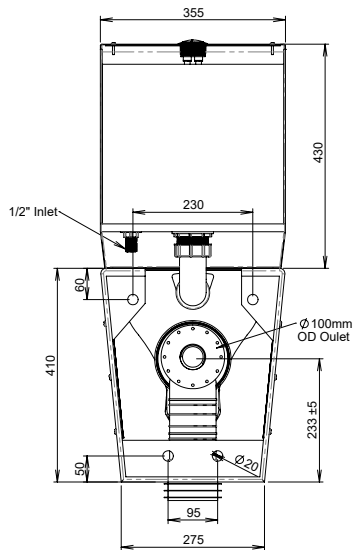
MODEL PTS Rear Elevation
