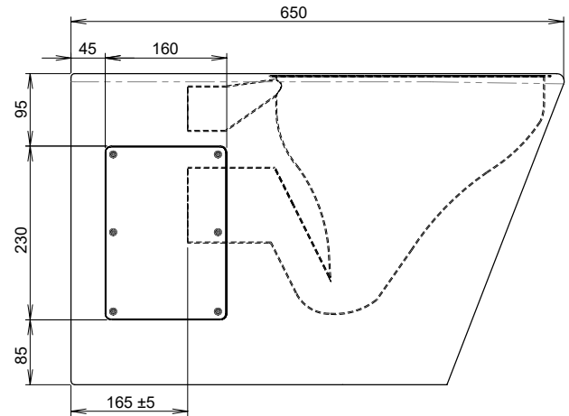
MODEL PC Side Elevation
