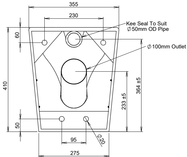
MODEL PC Rear Elevation
