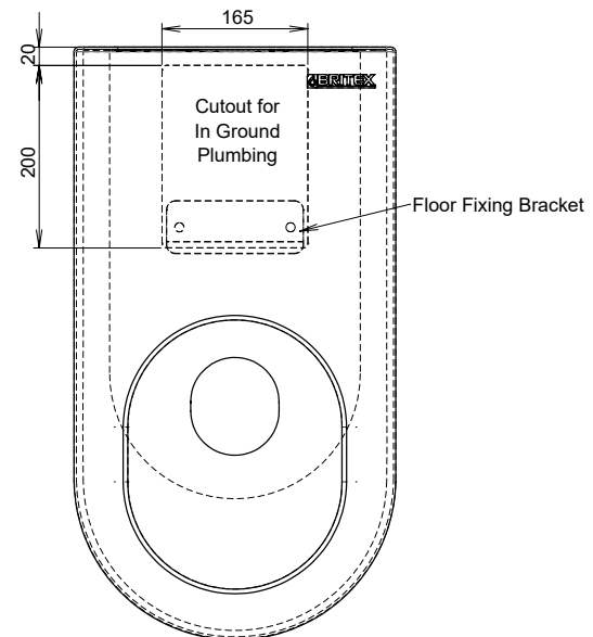
MODEL PC Plan
