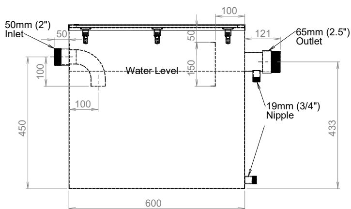
MODEL OSST Side Elevation
