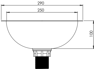
MODEL HBH3 Front Elevation
