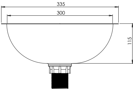
MODEL HBH2 Front Elevation
