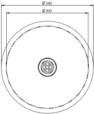
MODEL HBH2 Plan
