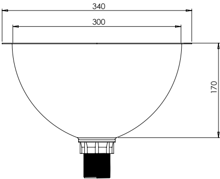
MODEL HBH2 Front Elevation
