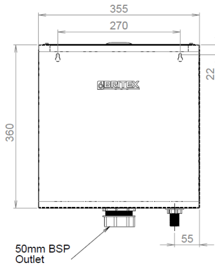
MODEL FCD Front Elevation
