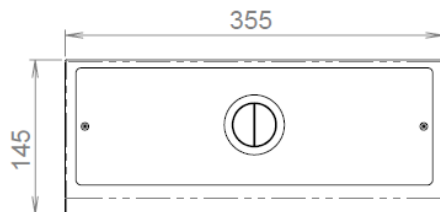
MODEL FCD Plan
