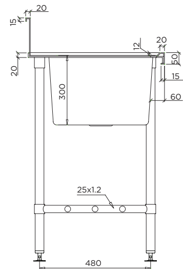
MODEL BT-SSB-618-R Section
