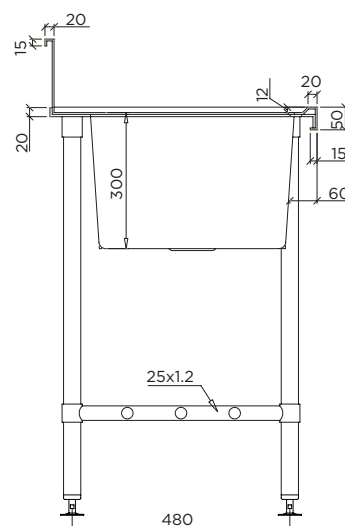
MODEL BT-SSB-615-R Section
