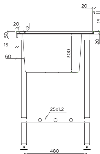
MODEL BT-SSB-615-L Section
