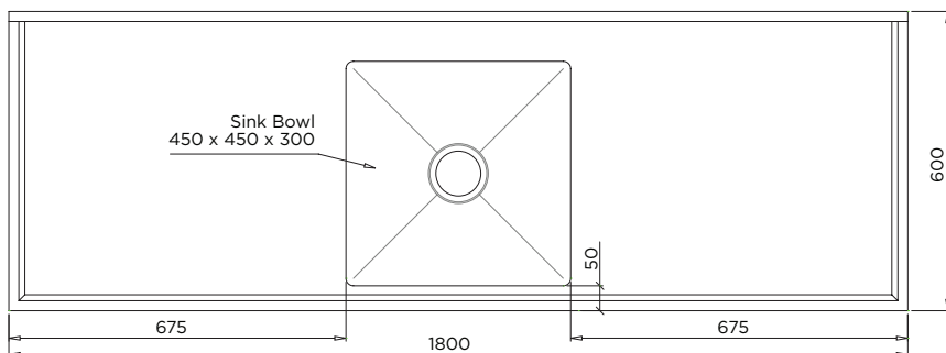
MODEL BT-SSB-618-C Plan
