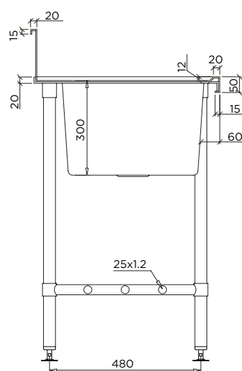
MODEL BT-SSB-618-C Section
