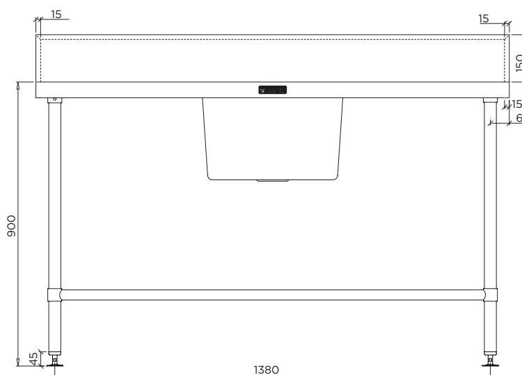
MODEL BT-SSB-615-C Front Elevation
