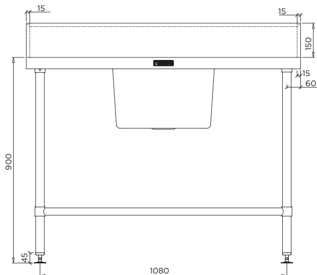
MODEL BT-SSB-612-C Front Elevation
