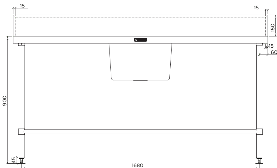
MODEL BT-SSB-618-C Front Elevation
