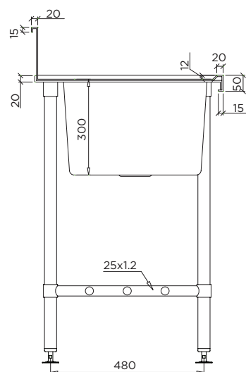
MODEL BT-SSB-615-C Section
