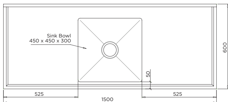
MODEL BT-SSB-615-C Plan
