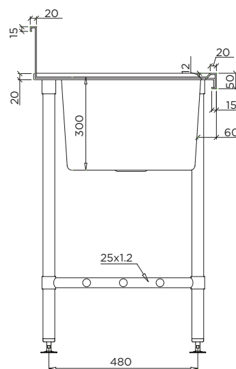
MODEL BT-SSB-612-C Section
