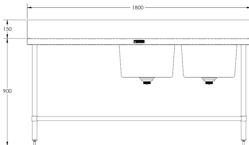
MODEL BT-DSB-618-R Front Elevation
