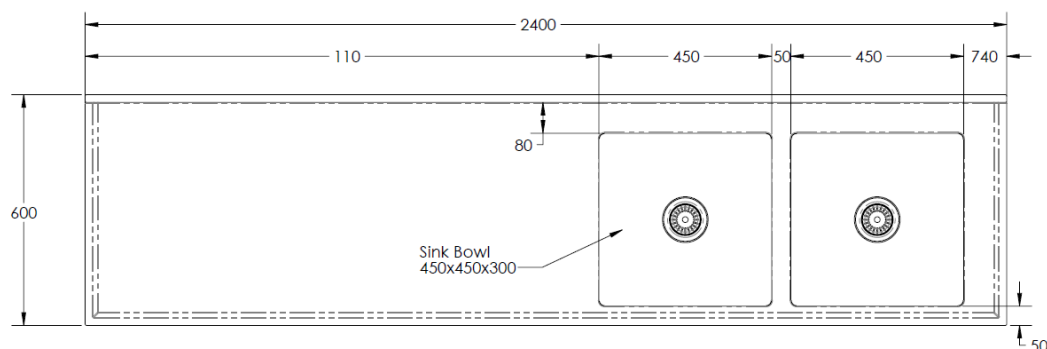
MODEL BT-DSB-624-R Plan
