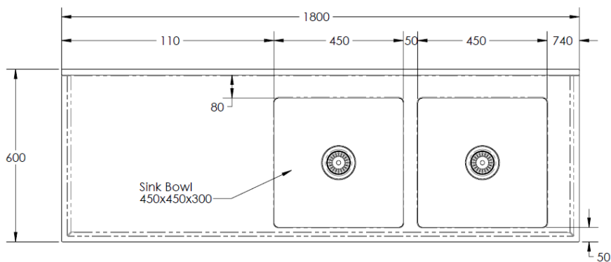
MODEL BT-DSB-618-R Plan
