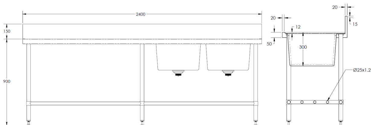
MODEL BT-DSB-624-R Front Elevation and Section
