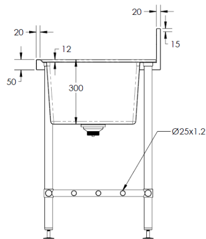
MODEL BT-DSB-618-R Section
