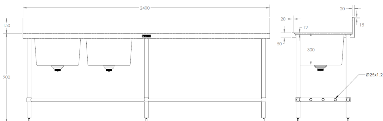
MODEL BT-DSB-624-L Front Elevation and Section
