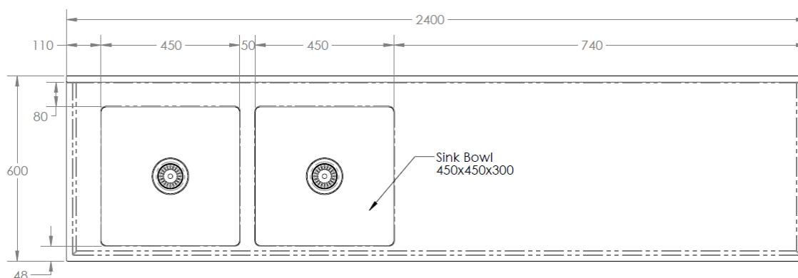
MODEL BT-DSB-624-L Plan
