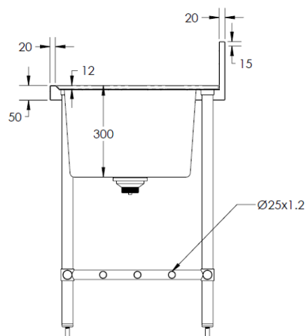
MODEL BT-DSB-618-L Section
