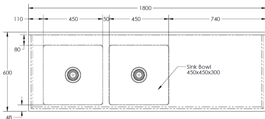
MODEL BT-DSB-618-L Plan
