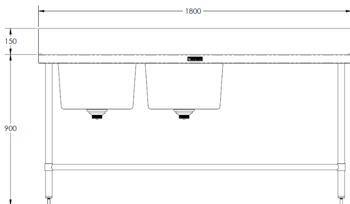
MODEL BT-DSB-618-L Front Elevation
