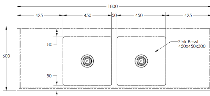
MODEL BT-DSB-618-C Plan
