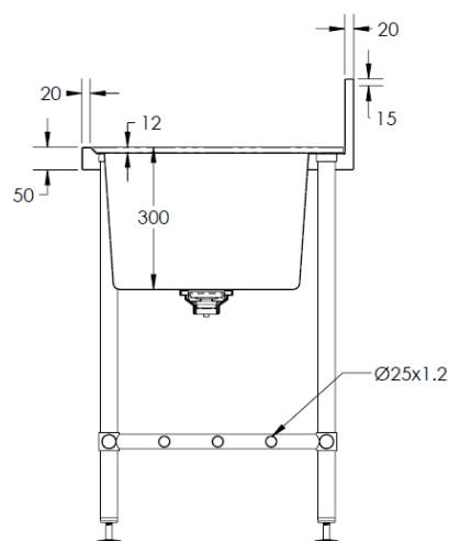
MODEL BT-DSB-618-C Section
