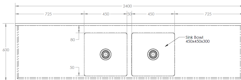
MODEL BT-DSB-624-C Plan
