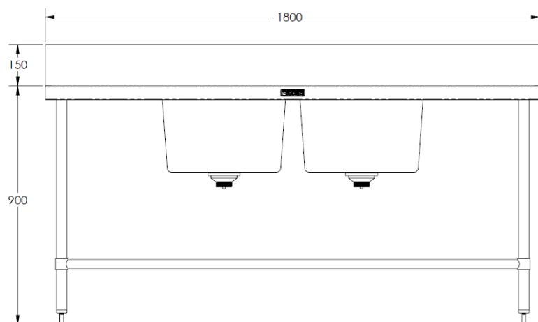
MODEL BT-DSB-618-C Front Elevation
