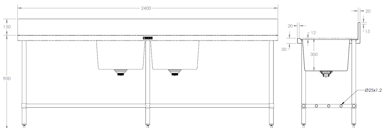
MODEL BT-DSB-624-C Front Elevation and Section
