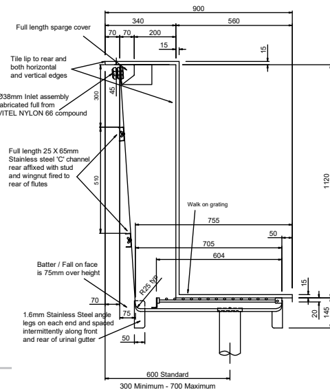
TYPICAL SECTION (Rear entry shown)
