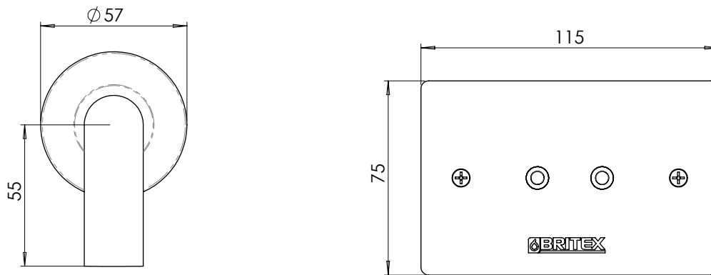
MODEL TW-WMS165 Front View
