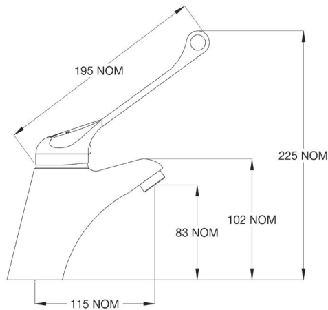
MODEL TW-MIX-L Side View
