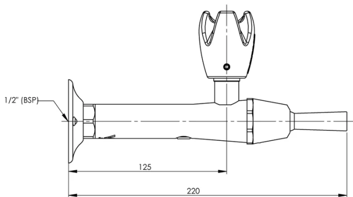
MODEL TW-DL90R Side View
