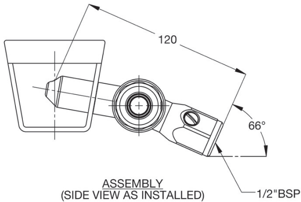
MODEL TW-DL45 Side View
