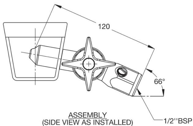
MODEL TW-DC45 Side View
