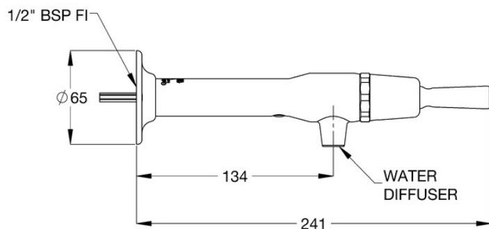
MODEL TW-BF-L90 Side View
