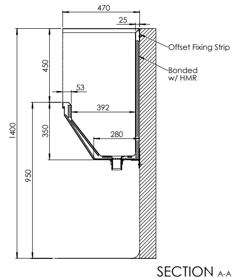
MODEL TST Section View
