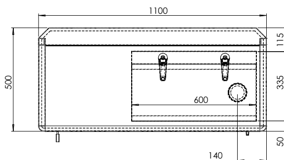
MODEL TP9P11-TW-9101 Plan
