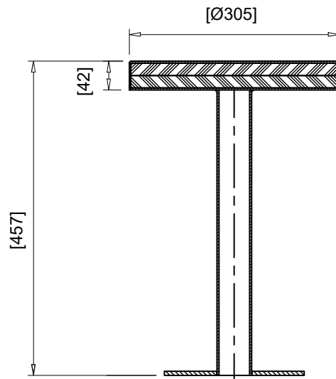
MODEL STLF Front Elevation
