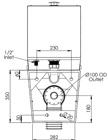
MODEL PTSCC Rear View
