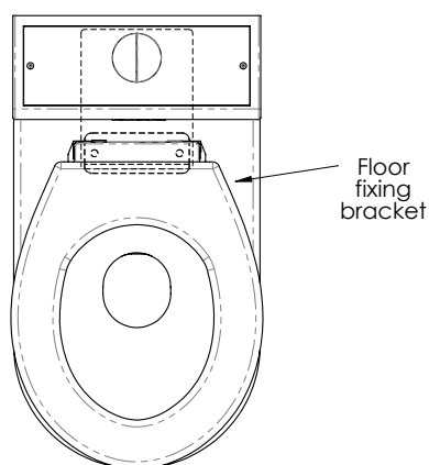
MODEL PTSCC Plan View
