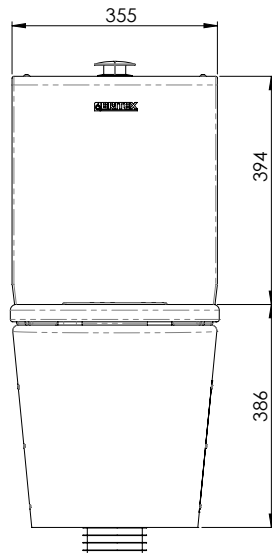
MODEL PTSCC Front View
