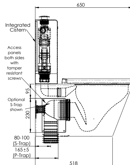
MODEL PTSCC Side View
