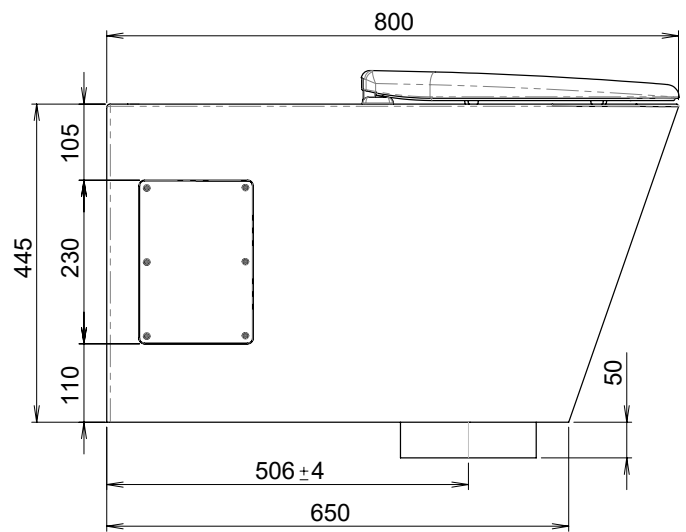
MODEL PLDD Side View
