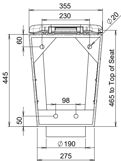
MODEL PLDD Rear View
