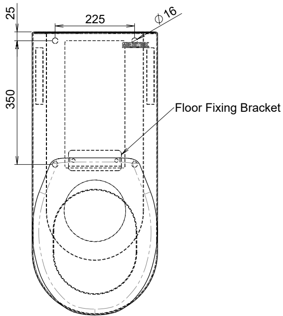
MODEL PLDD Plan
