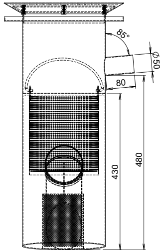
MODEL OSCBT-V Front Elevation
