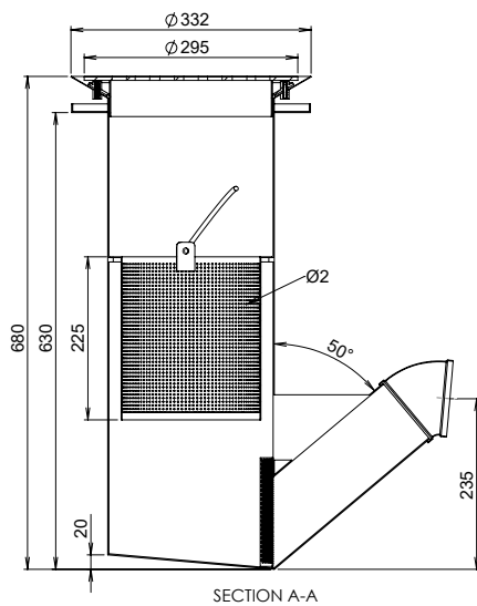
MODEL OSCBT-V Side Elevation
