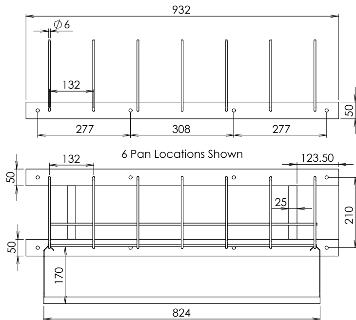
MODEL LPBR Front View
