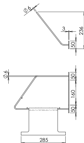
MODEL LPBR Side View
