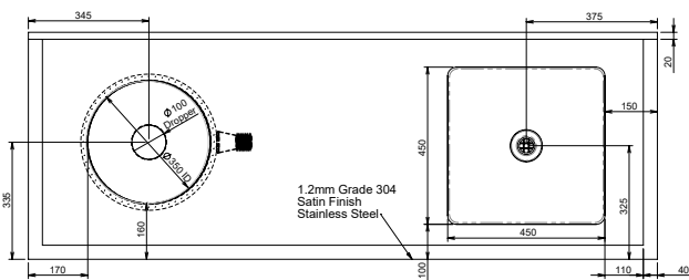
MODEL LDUS-A Plan View
