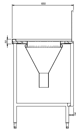
MODEL LDUS-A Section View
