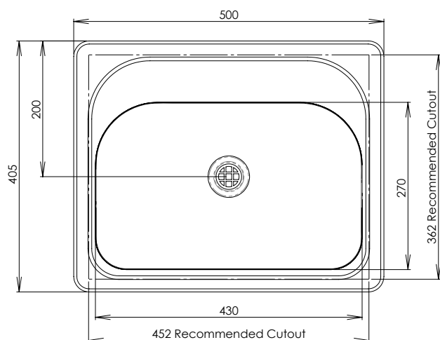
MODEL SPBO Plan View
