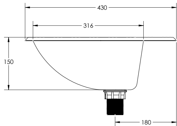
MODEL HBRE Side View
