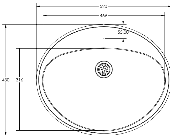
MODEL HBRE Plan View
