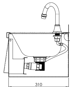
MODEL HBKOC Section View
