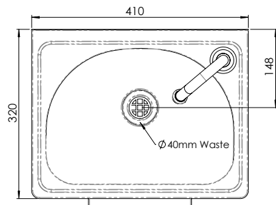
MODEL HBKOC Plan View
