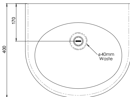
MODEL HBGU Plan View
