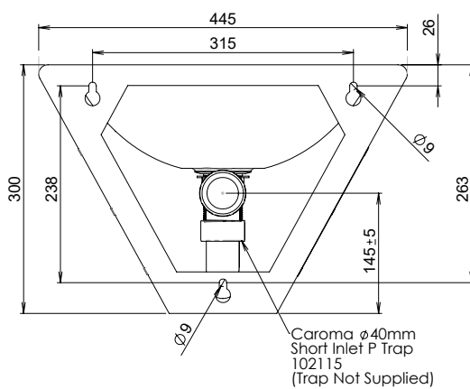
MODEL HBGU Plan View
