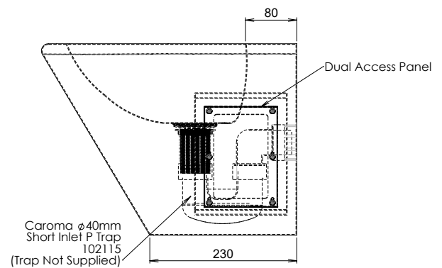
MODEL HBGU Side View
