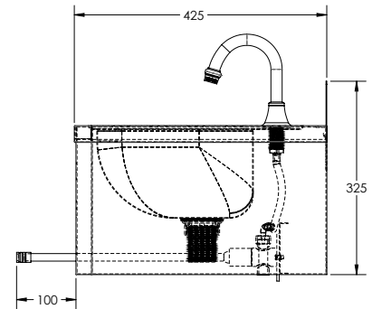
MODEL HBFWs Side View
