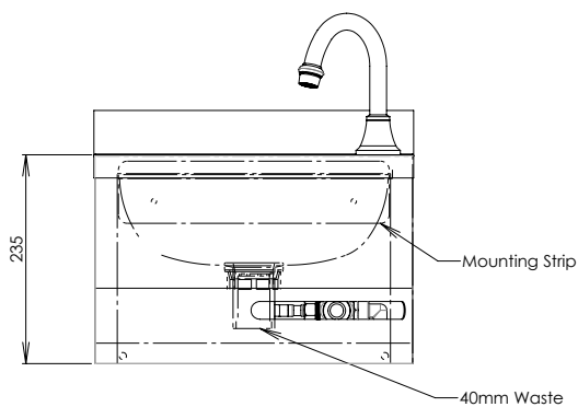
MODEL HBFWR Front View
