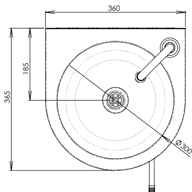
MODEL HBFWR Plan View
