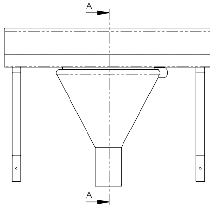
MODEL FLF2 Front Elevation
