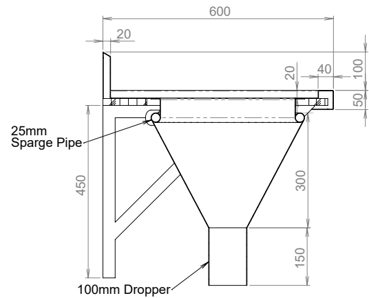
MODEL FLF2 Section View
