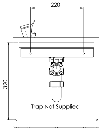
MODEL DVR Rear Elevation
