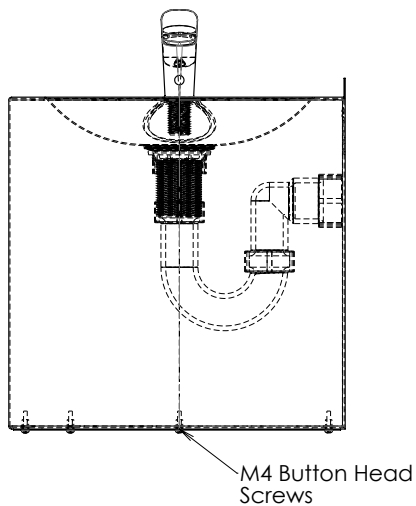
MODEL DVR Side View
