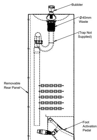
MODEL DSSR-H Section
