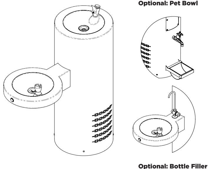
MODEL DSRR-2-TW-BF-HF-PB Isometric View
