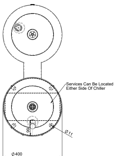
MODEL DSRR-2 Plan
