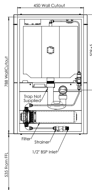
MODEL DHFBBF-IW-VR Section View
