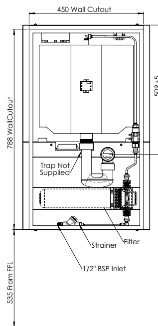
MODEL DHFBF-IW-B Section View
