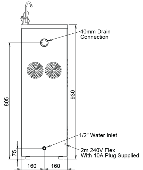
MODEL DFW4 Back View
