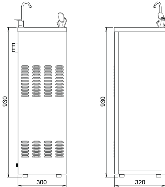
MODEL DFW4 Front and Side View
