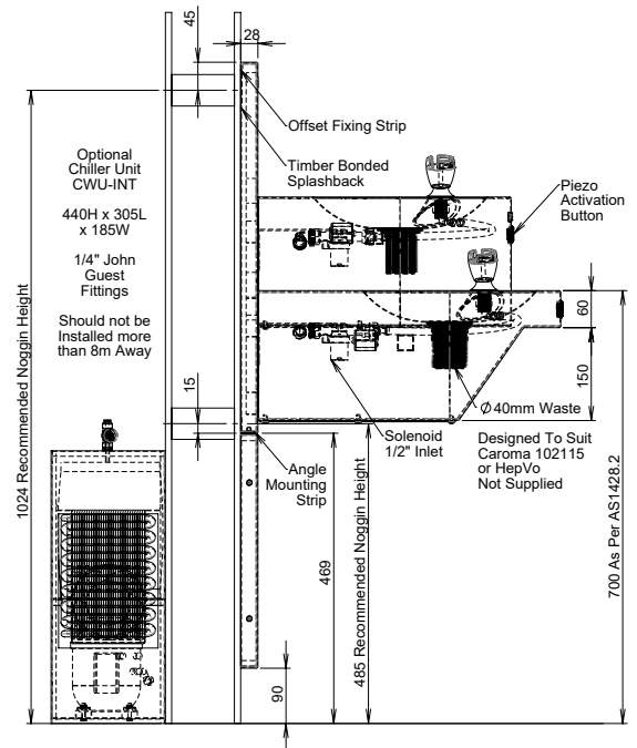
MODEL DDR2 Side View
