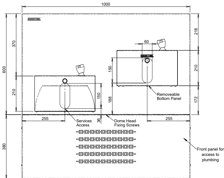
MODEL DDR2 Front View
