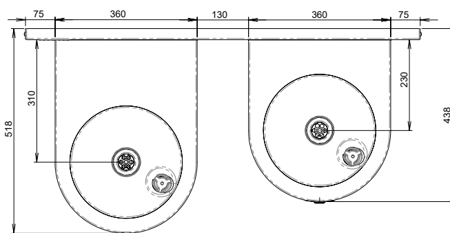
MODEL DDR2 Plan View
