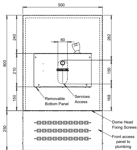
MODEL DDR1-S Front View
