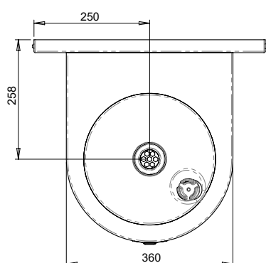
MODEL DDR1-S Plan View
