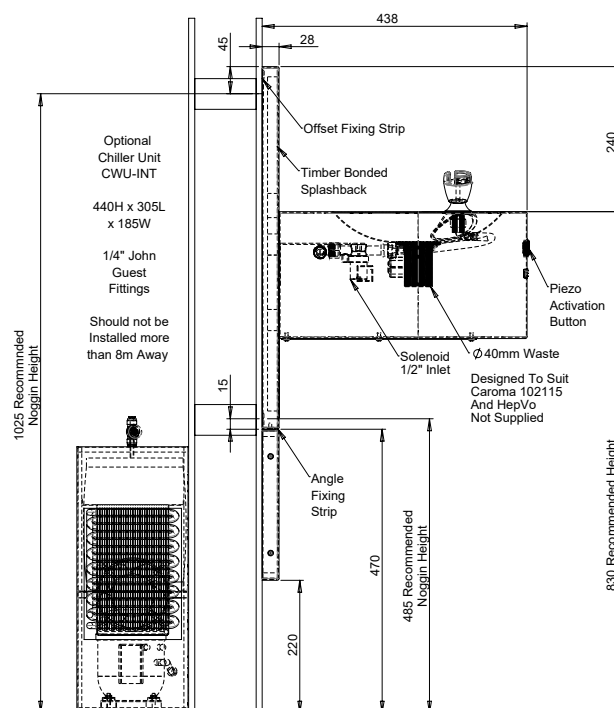
MODEL DDR1-S Side View
