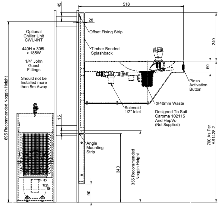
MODEL DDR1-D Side View
