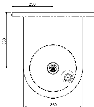
MODEL DDR1-D Plan View
