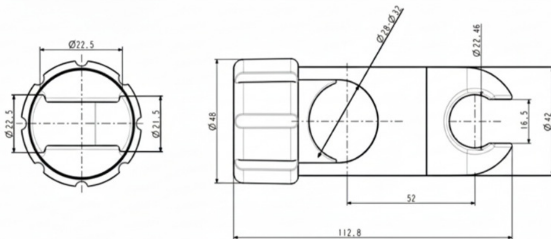
MODEL BTR-01-051 Side and Plan Elevation
