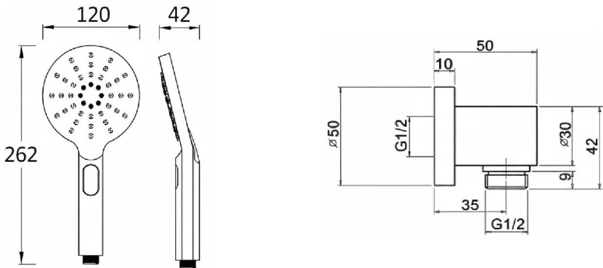
MODEL BTR-01-051 Side and Plan Elevation
